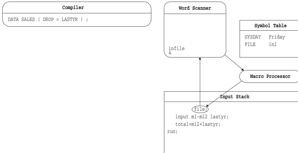
Figure 2.9 The Macro Processor Examines &FILE
